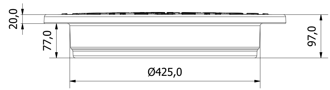
Front
